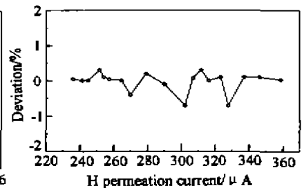
Fig. 5 Change of the deviation of the result measured from the input signal with hydrogen permeation rate
