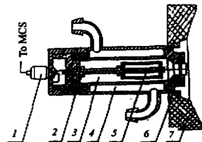
Fig. 1 Schematic diagram of the outward attached electrochemical sensor
