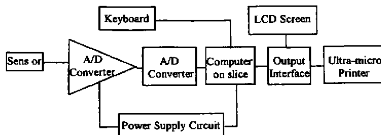
Fig. 2 Schematic diagram of the MCS and the periphery attachment
