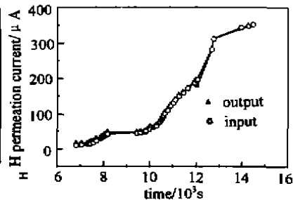
Fig. 4 The relationship between the signals input into and output from MCS
