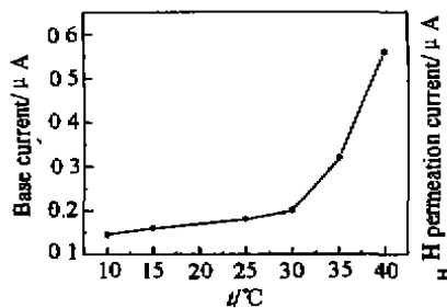
Fig. 3 The effect of temperature on base current
