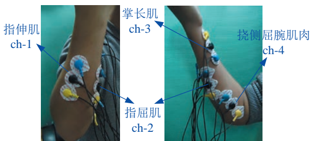
图 1 表面肌电电极布置 (ch- l 表示第 l 通道, l = 1, 2, 3, 4 ) Fig.1 The placement of the sEMG electrodes (ch- l represents the l -th electrode channel, l = 1, 2, 3, 4 )
