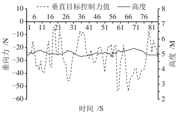
图 5 垂向推进器控制的高度变化曲线 Fig.5 Height curve with vertical thruster control
